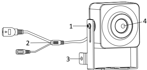
Figure 1-1 Overview of Type I Mini Camera
