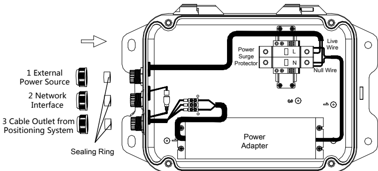
Figure 2-17 Cable Connection of Junction Box
