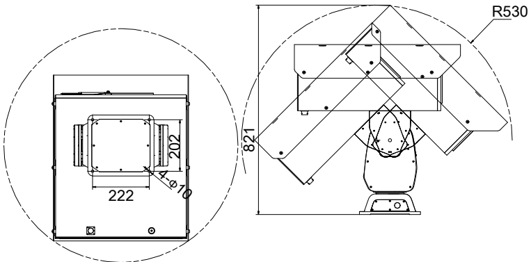
Figure 2-2 Large-sized Housing Positioning System Dimensions (1)
