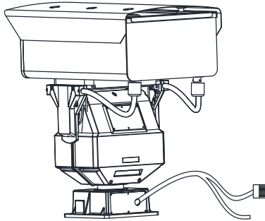
Figure 2-13 Route the Cables
