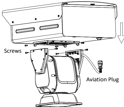
Figure 2-9 Connect the Housing and the Positioning System Base
