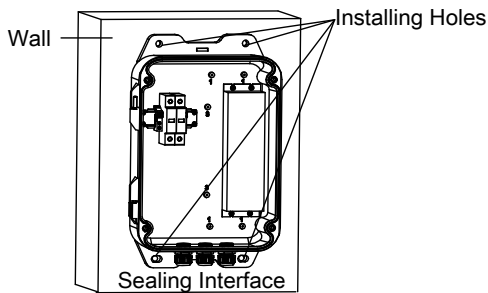
Figure 2-14 Fix the Junction Box
