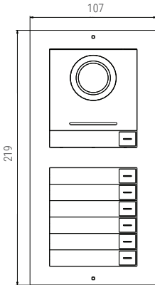
Dual Modules Surface Mounting
