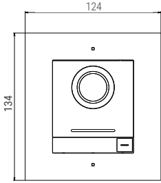
Single Module Flush Mounting
