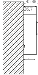
Single Module Surface Mounting
