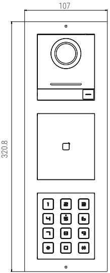
Three Modules Surface Mounting
