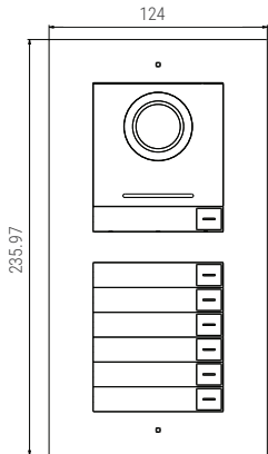
Dual Modules Flush Mounting
