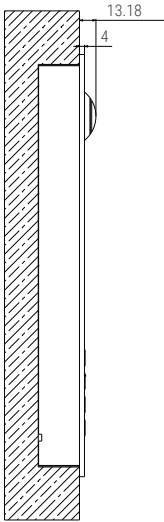
Three Modules Flush Mounting
