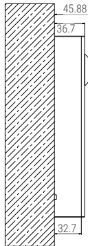
Dual Modules Surface Mounting
