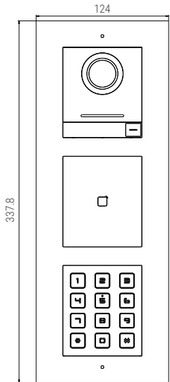
Three Modules Flush Mounting
