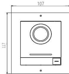
Single Module Surface Mounting
