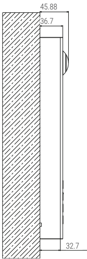
Three Modules Surface Mounting
