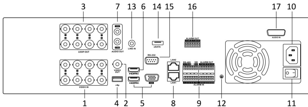
Figure 1-26 Rear Panel of DS-9000HUHI-K8 (with 8 Video Inputs)
