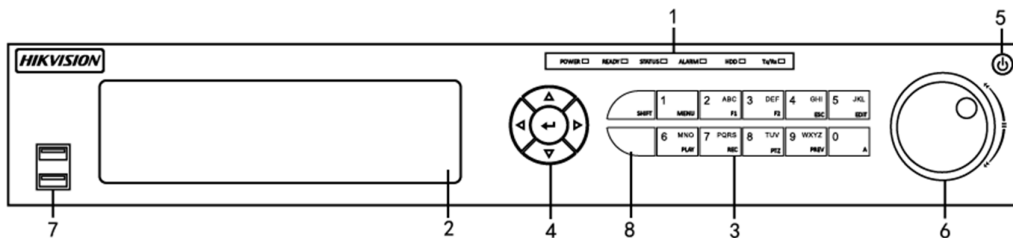
Figure 1-2 Front Panel
