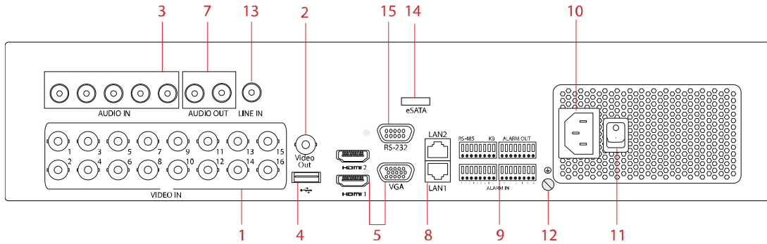
Figure 1-25 Rear Panel of DS-7300HUHI/HTHI-K4, iDS-7316HUHI-K4/16S, and DS-7316HTI-K4
