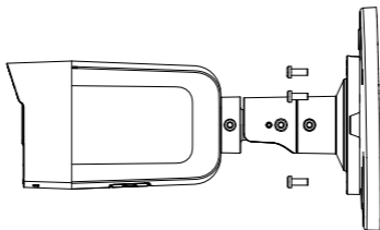
Figure 2-6 Fix the Camera on Junction Box's Cover
