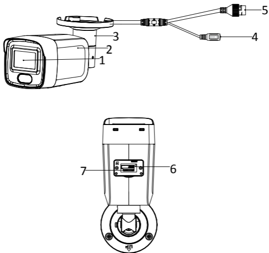
Figure 1-1 Bullet Camera Overview
