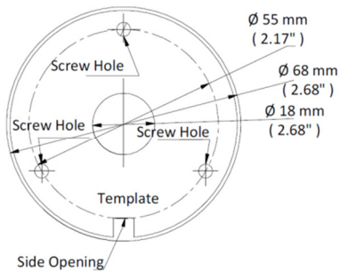
Figure 2, Drill Template
