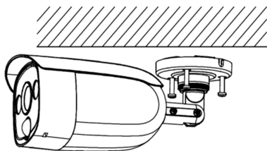
Figure 3, Fix the Camera to the Ceiling
