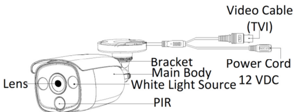
Figure 1, Camera Overview
