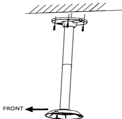
Figure 2-10 Install the Bracket
