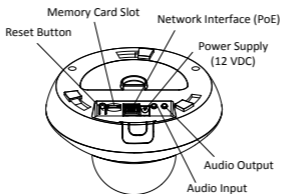
Figure 1-4 Interfaces of Type II Camera
