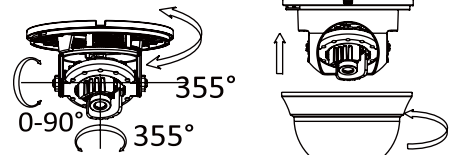
Figure 2-8 3-axis Adjustment & Lower Dome
