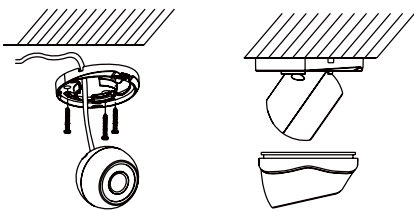
Figure 2-2 Fix the Mounting Base and the Camera 6. Adjust the camera according to the figure below to get an optimum angle.
