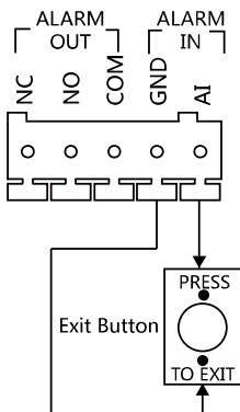
Figure 3-4 Exit Button Wiring
