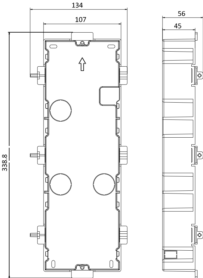
DS-KD-ACF3/Plastic
