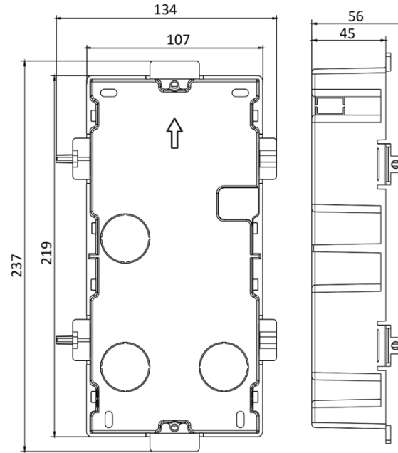
DS-KD-ACF2/Plastic
