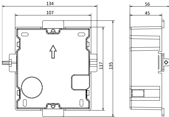
DS-KD-ACF3/Plastic
