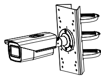
PM Vertical Pole Mount
